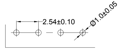
Recommened PCB Layout
