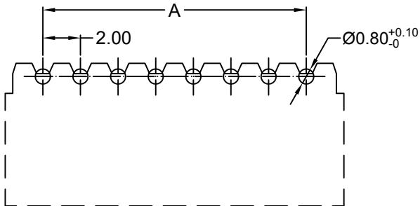
Conn.line Recommended P.C.B Layout General Tolerance±0.05
