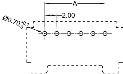
Recommended P.C.B Layout General Tolerance \pm 0.05
